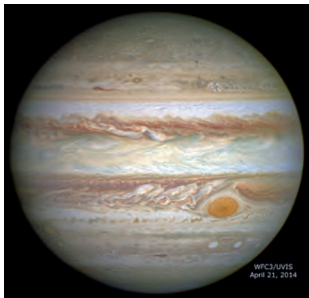
2014 WFC3/UVIS
